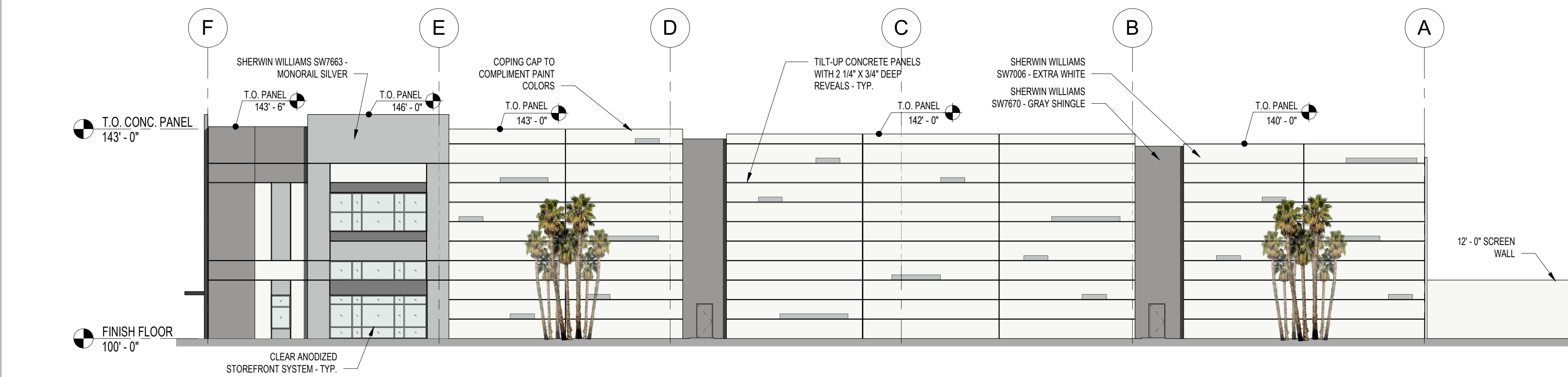
3 EAST ELEVATION A2 1/16" = 1'-0"
