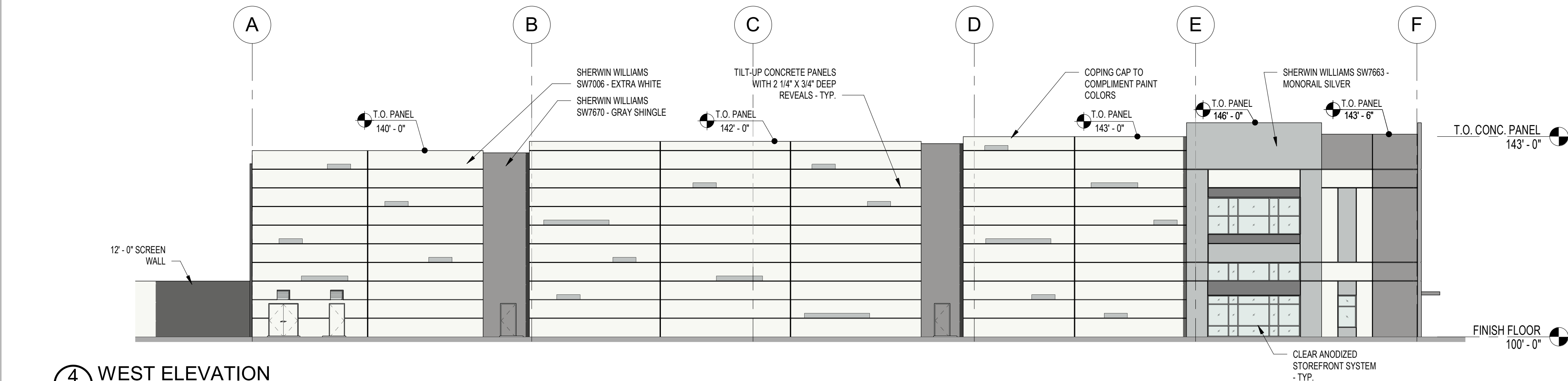
4 WEST ELEVATION A2 1/16" = 1'-0"
