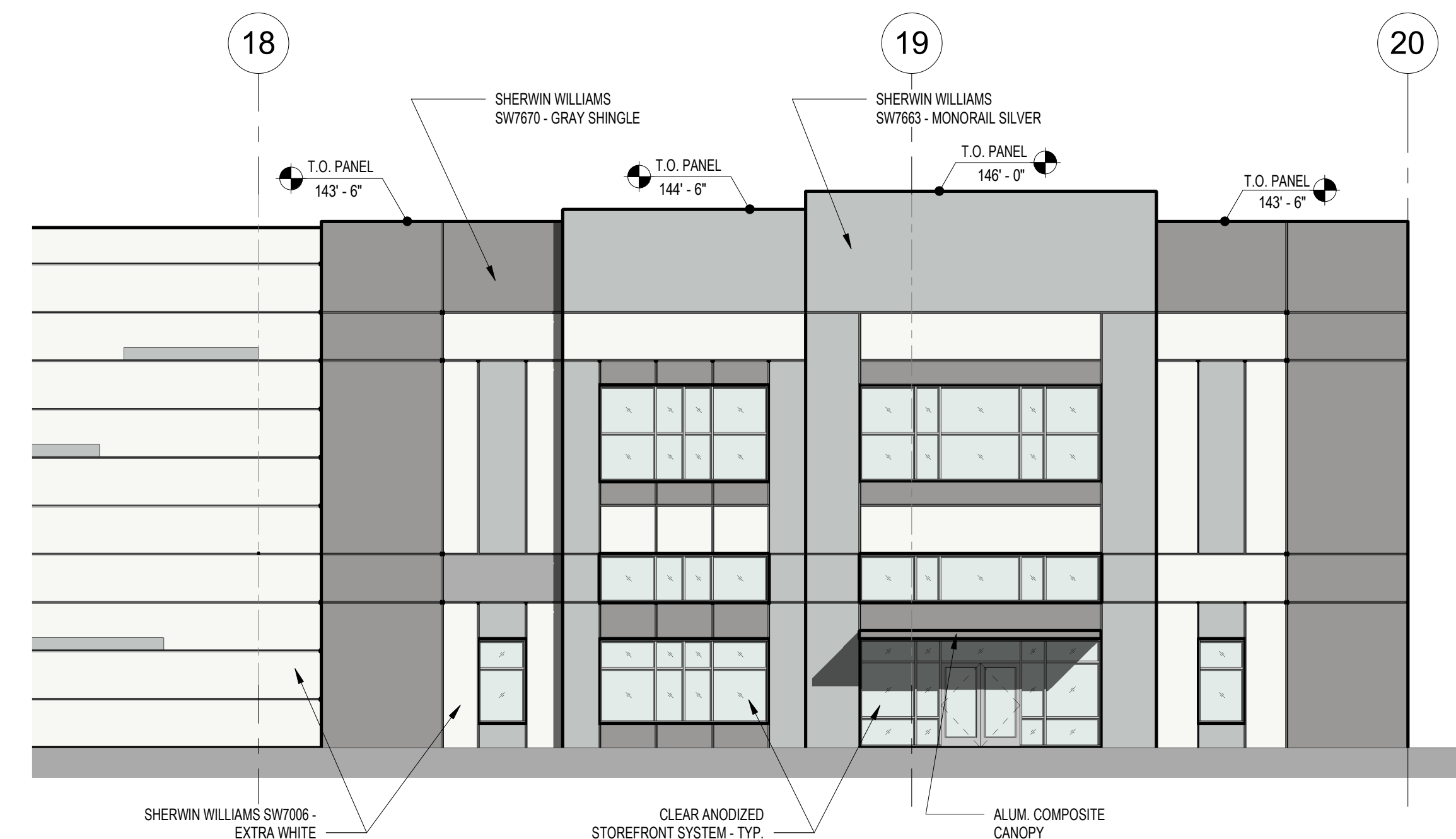
5 ENLARGED ENTRY ELEVATION A2 1" = 10'-0"
