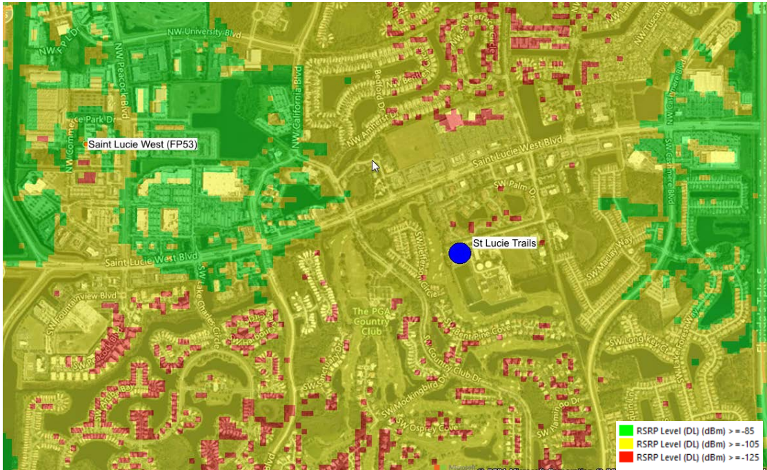
Signal level prediction plot, without proposed site St. Lucie Trails
