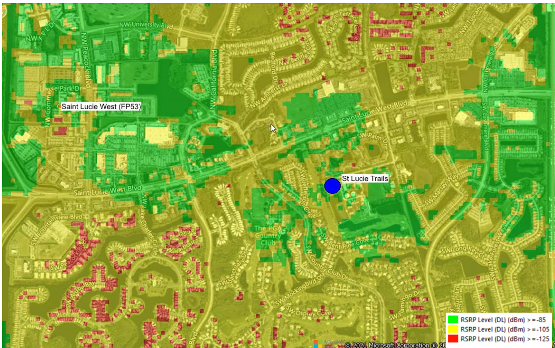
Signal level prediction plot, with proposed site St. Lucie Trails.
