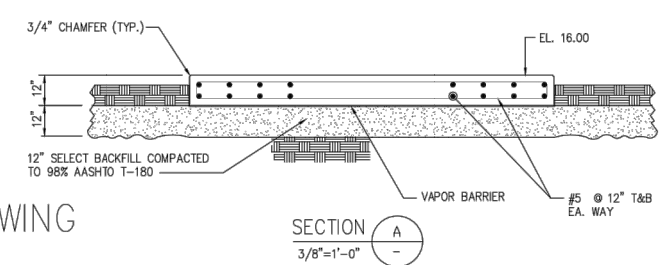
FUEL STORAGE TANK PLAN, FOUNDATION AND DETAILS
