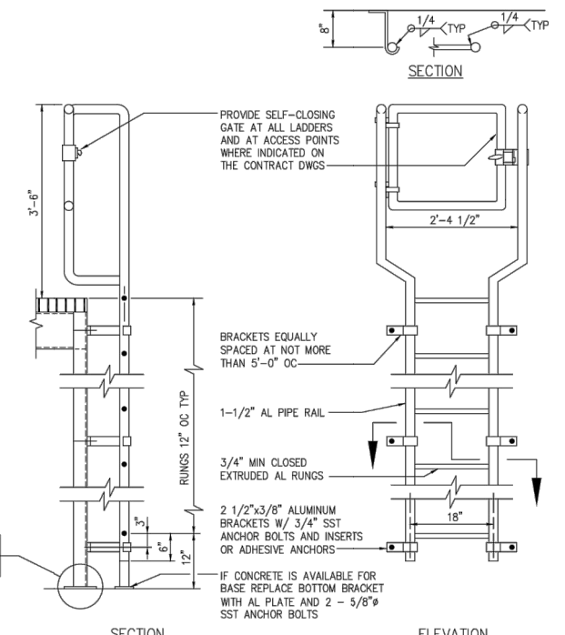
ALUMINUM LADDER
