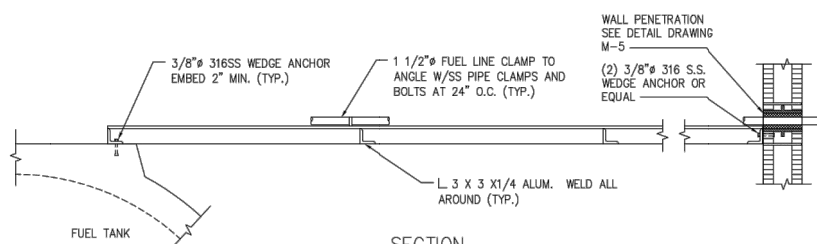
FUEL LINE SUPPORT DETAIL 3/4"=1'-0"
