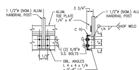
ELEV. SECTION
