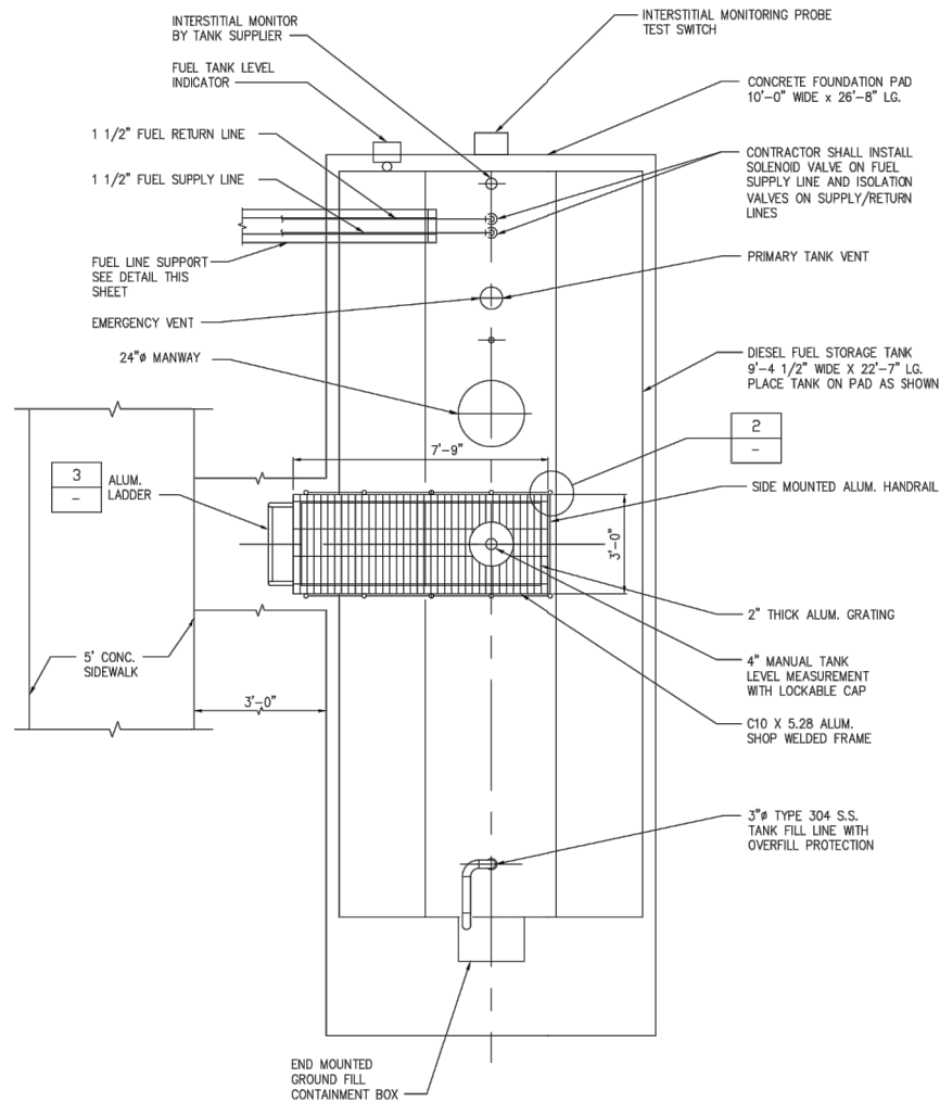
FUEL STORAGE TANK PLAN
