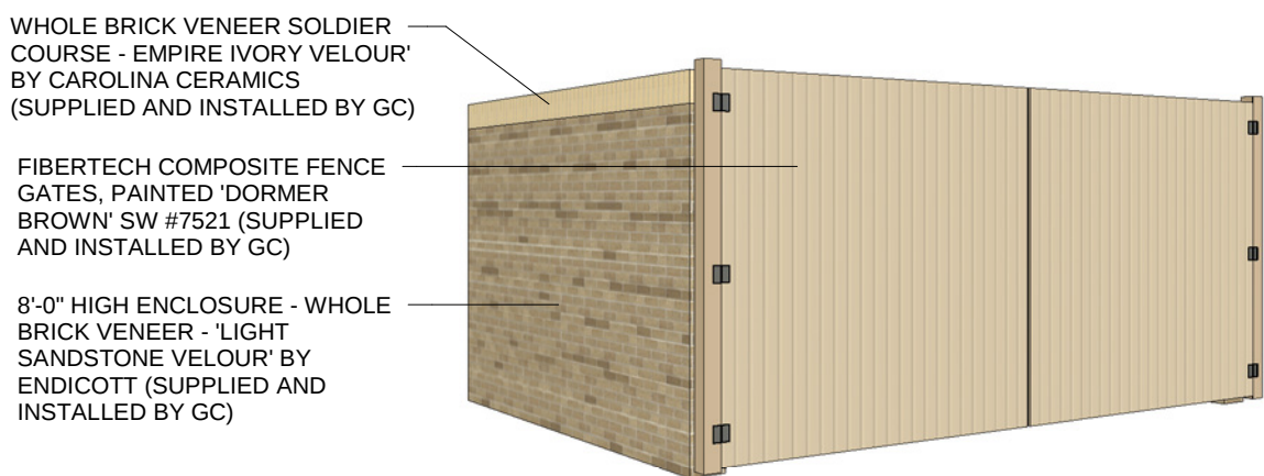
6 TRASH ENCLOSURE
