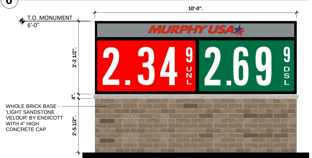
7 MONUMENT SIGN
