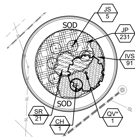
MEDIAN 3 SCALE 1"=30'-0"
