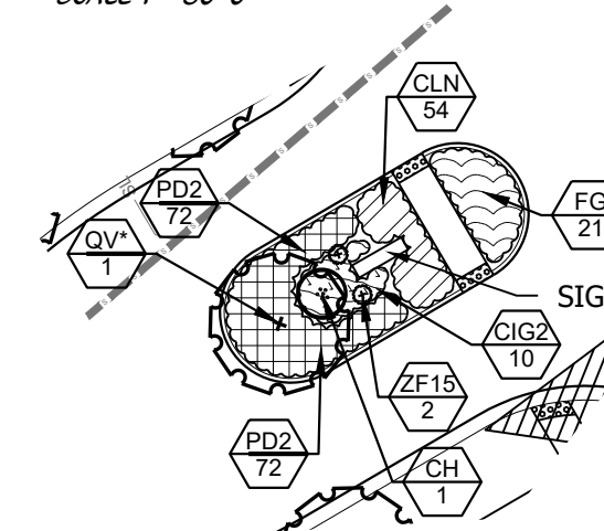
MEDIAN 8 SCALE 1"=30'-0"
