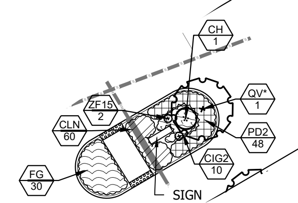
MEDIAN 4 SCALE 1"=30'-0"
