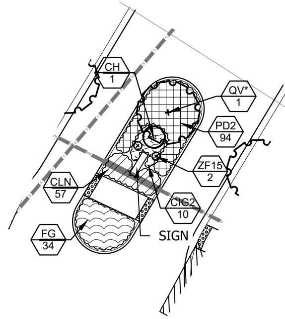
MEDIAN 2 SCALE 1"=30'-0"
