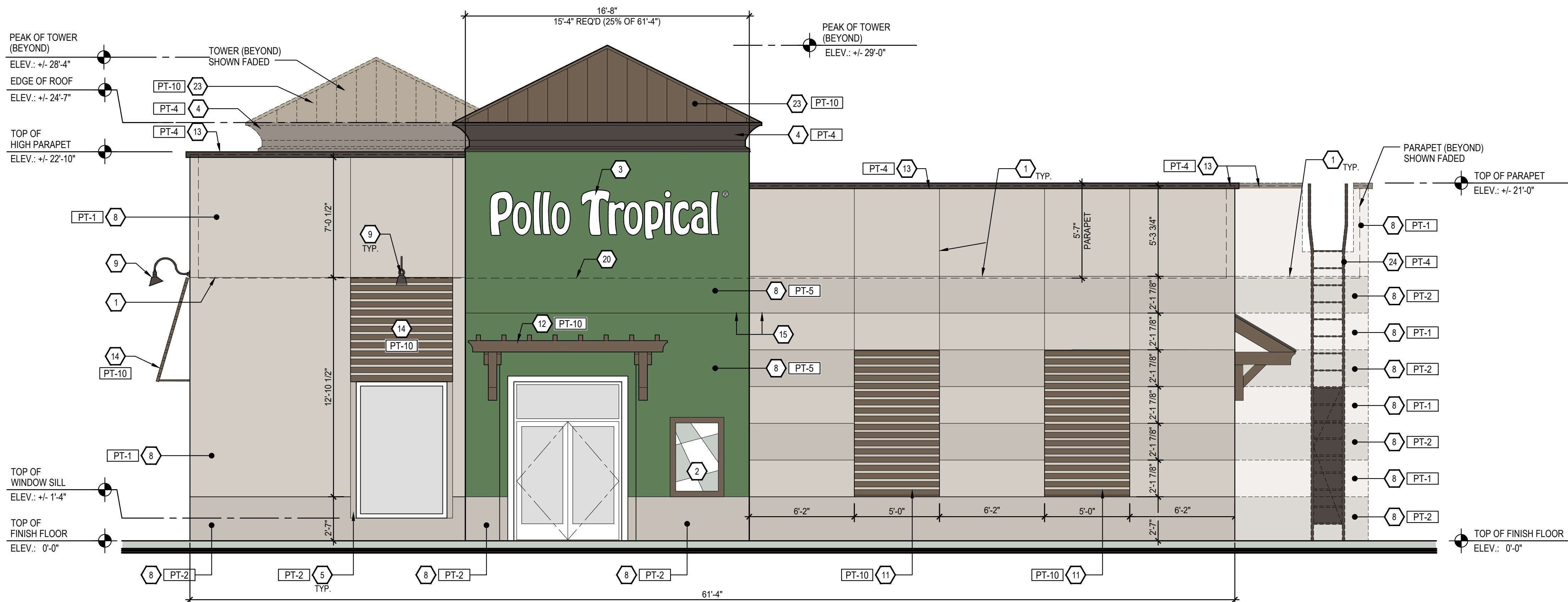
2 FRONT (WEST) EXTERIOR ELEVATION
