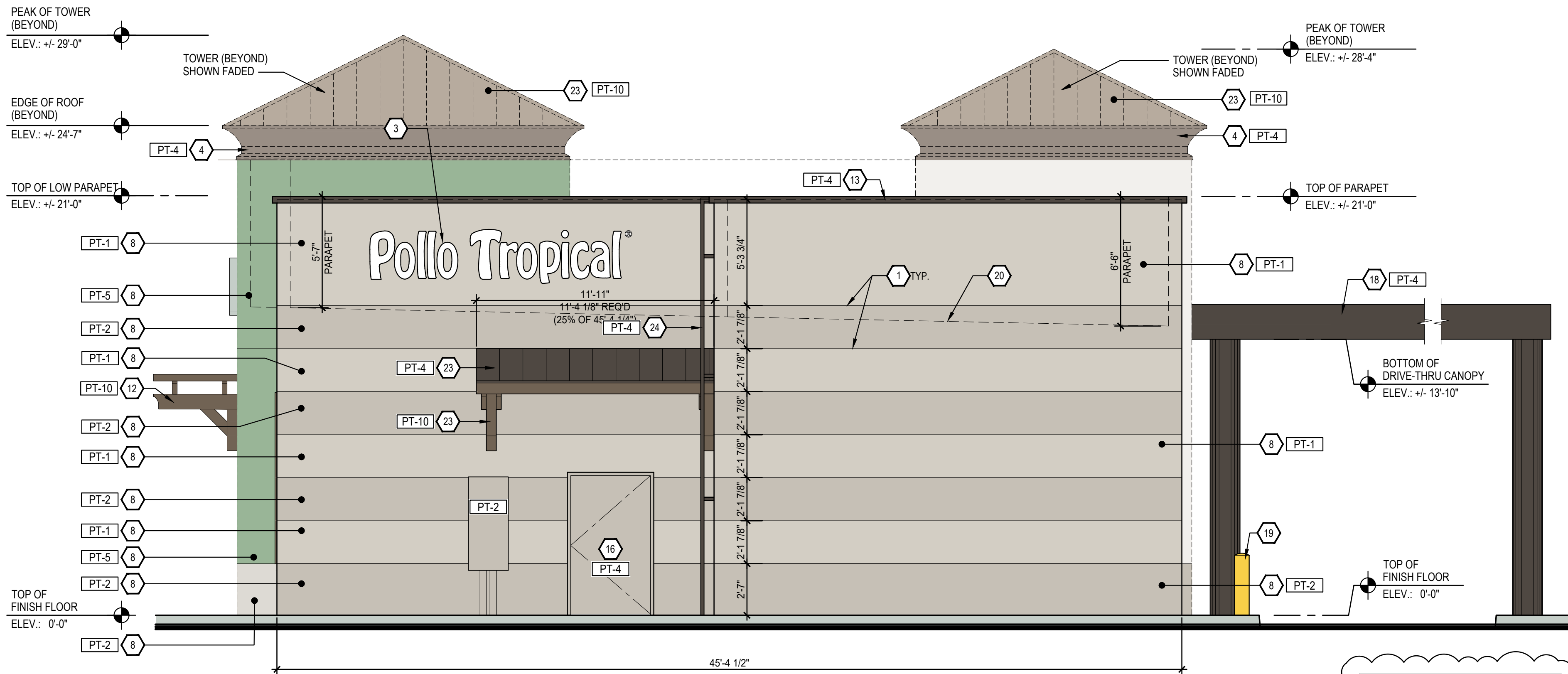
1 RIGHT (SOUTH) SIDE EXTERIOR ELEVATION
