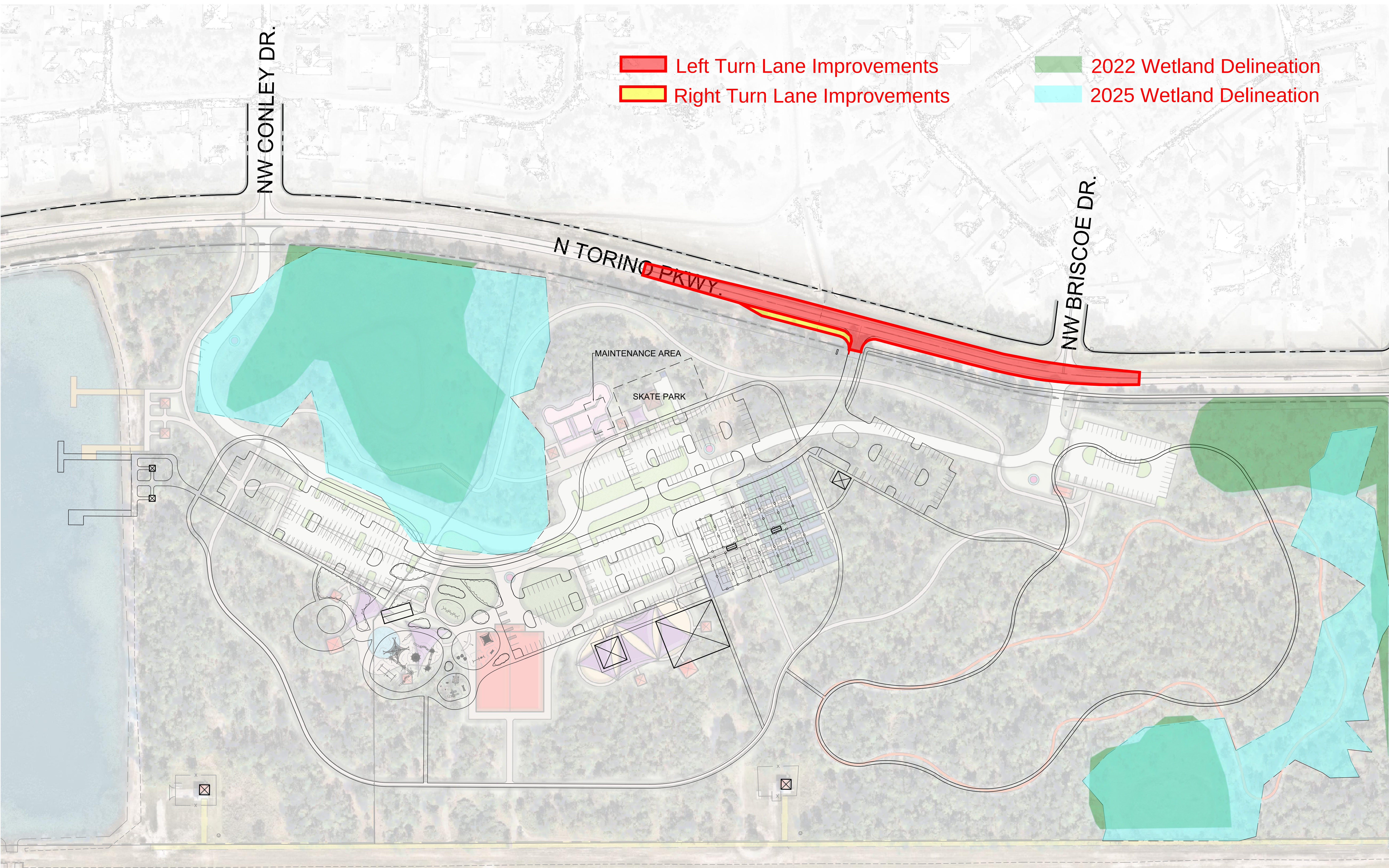
TORINO REGIONAL PARK PHASE 1 SINGLE ENTRANCE- OPTION 1A
