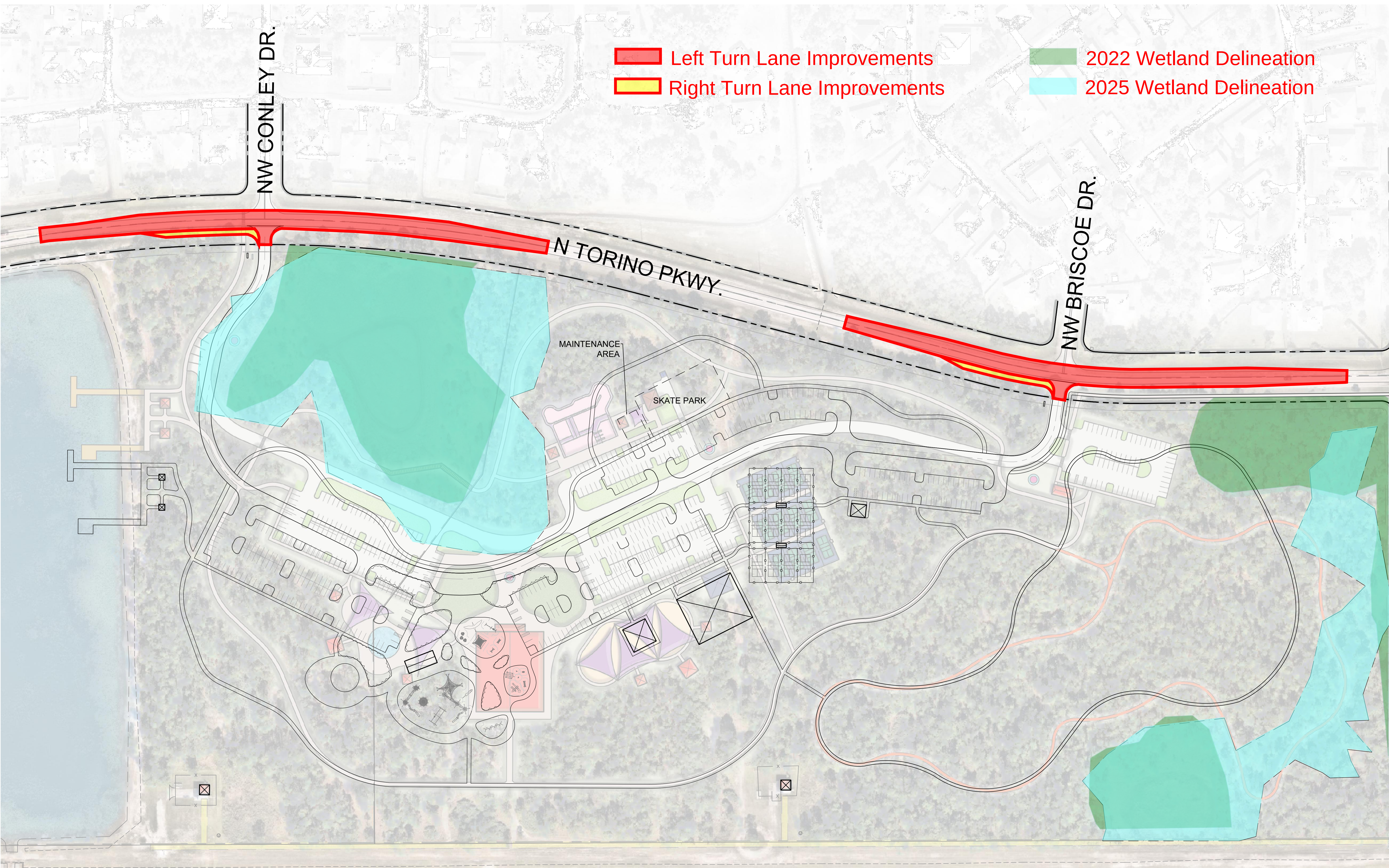
TORINO REGIONAL PARK PHASE 1 TWO ENTRANCES- OPTION 2
