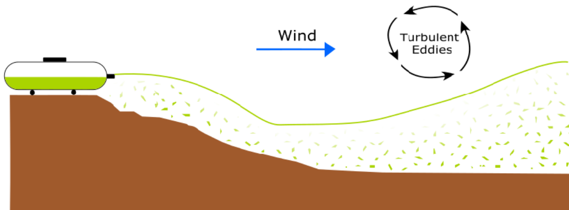
Figure 3.2 - Dense Gas Behavior
