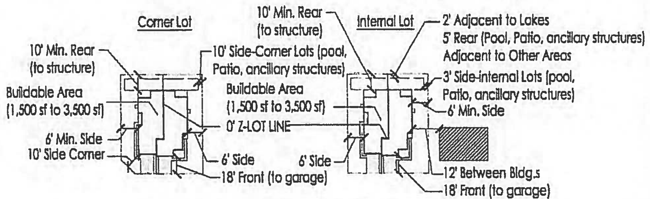
TYPICAL PAIRED VILLA LOT (PAIRED VILLA ATTACHED MIN. 118' LENGTH X MIN. 37.5' WIDTH)
