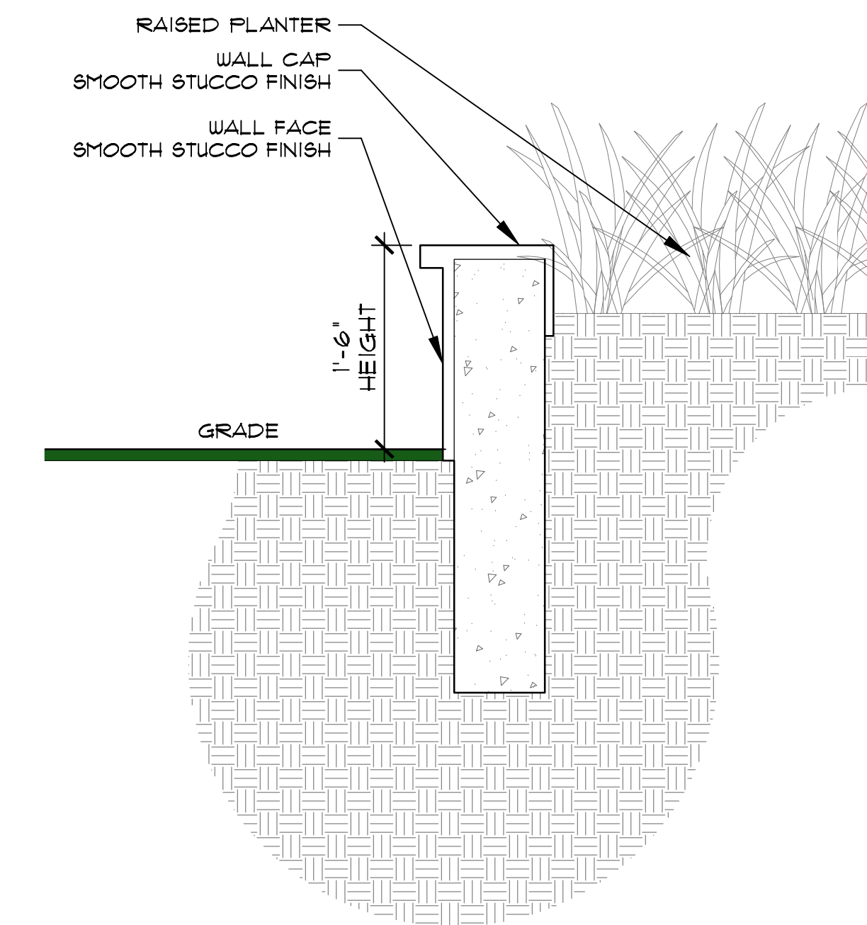
C RAISED PLANTER WALL H-2
