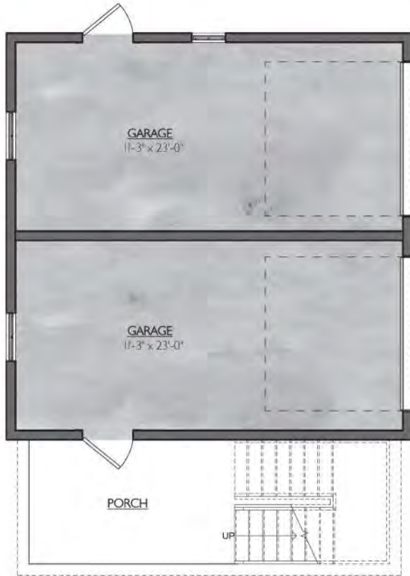
Main Floor Plan (576 sq ft)
