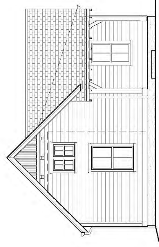
3 | 1 & 2 Bedroom Twin Elevations A200 1/8" = 1'-0"
