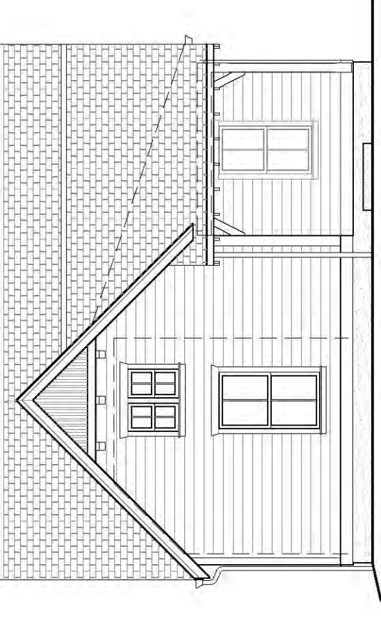
1 | 1 Bedroom Twin Elevations A200 1/8" = 1'-0"
