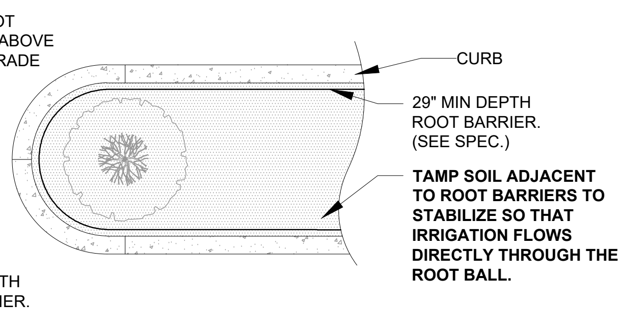
SPECIAL APPLICATIONS ROOT BARRIER DETAIL NOT TO SCALE
