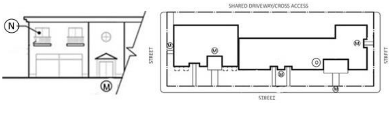
Figure 3-18: Building Elements (Activity Center & Village)
