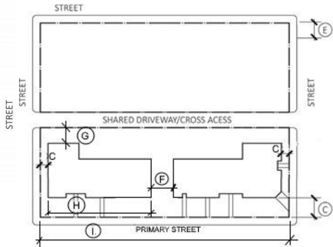
Figure 3-17: Building Placement (Activity Center)
