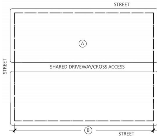
Figure 3-21: Lot Criteria (Activity Center)
