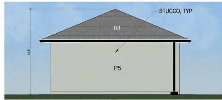
4 Left Elevation
