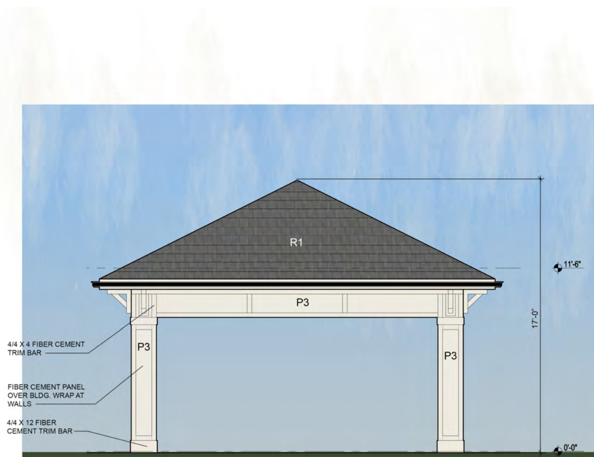
1 Typical Elevation
