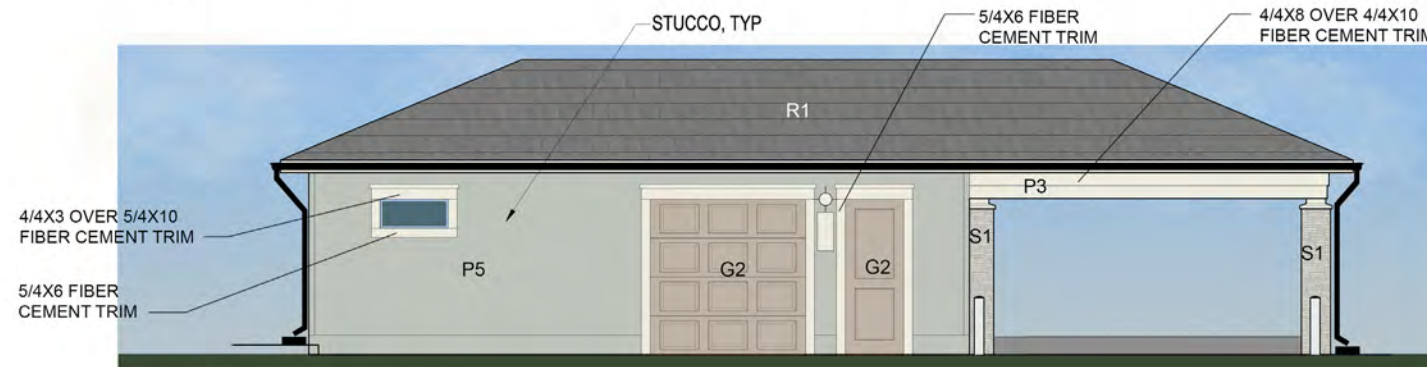
1 Front Elevation
