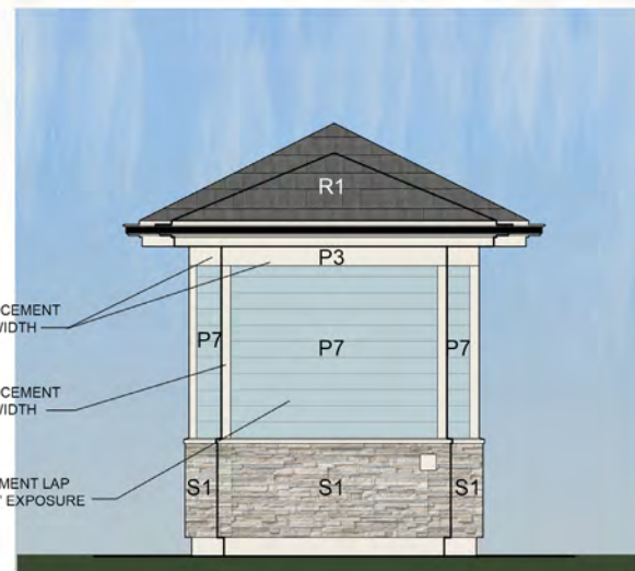
Rear Elevation
