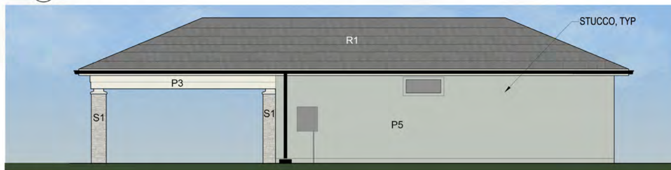
2 Rear Elevation
