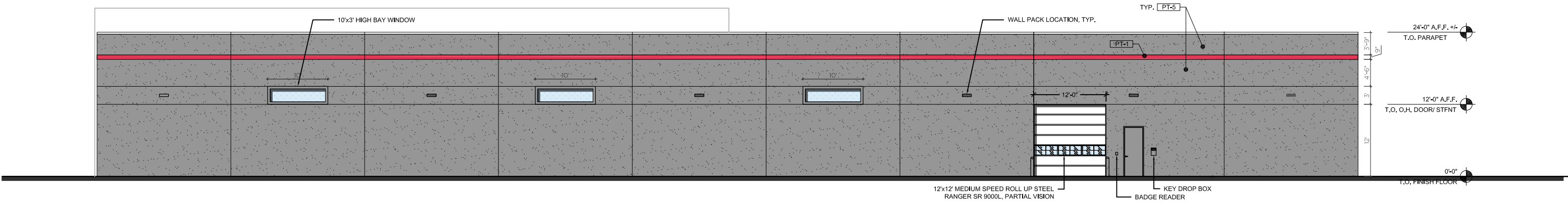
SOUTH ELEVATION
