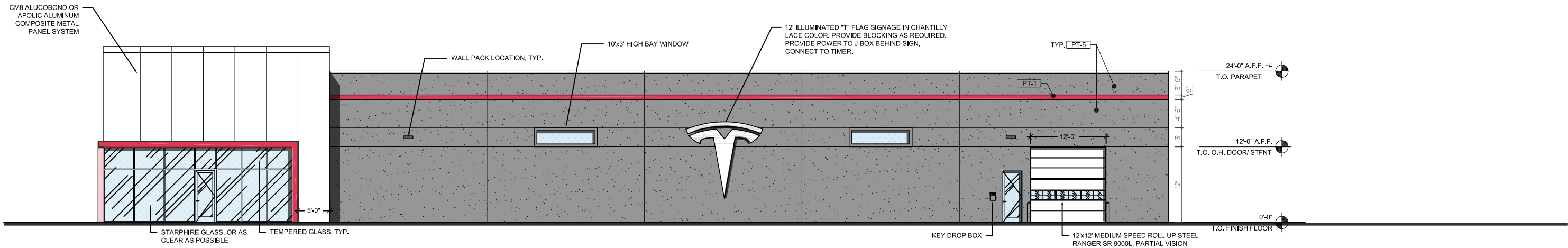
WEST ELEVATION
