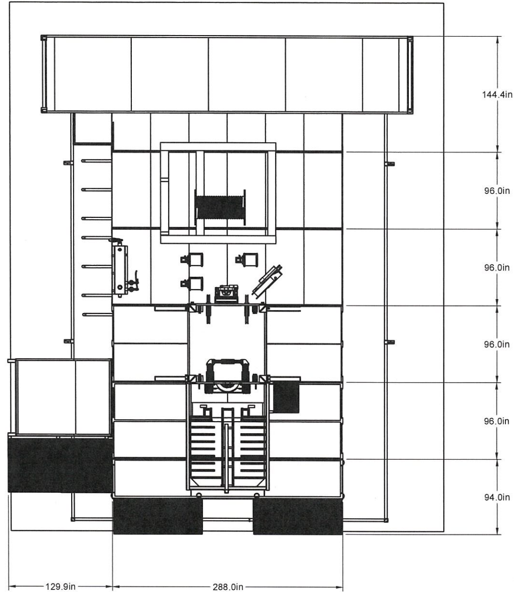
E6 RIG - TOP VIEW SCALE 1:120
